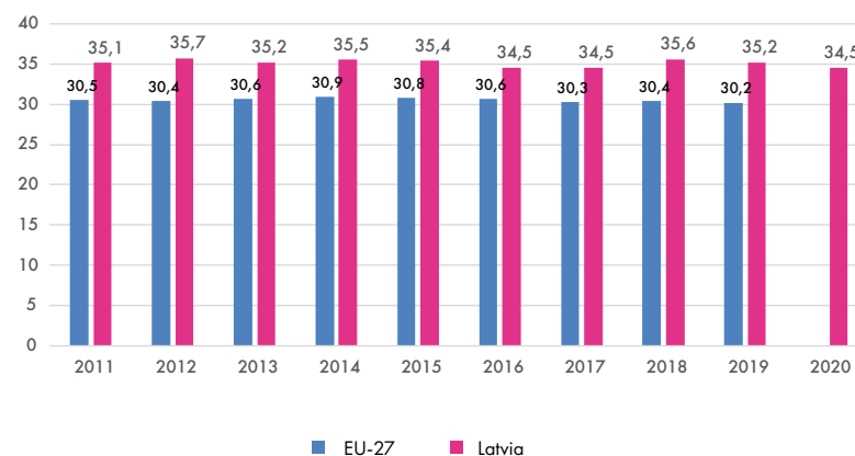
GINI COEFFICIENT
